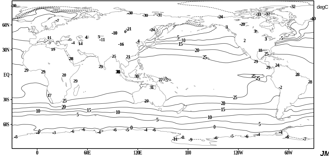
Sea surface temperature and sea ice surface temperature average (1981-2010) JMA March-May
