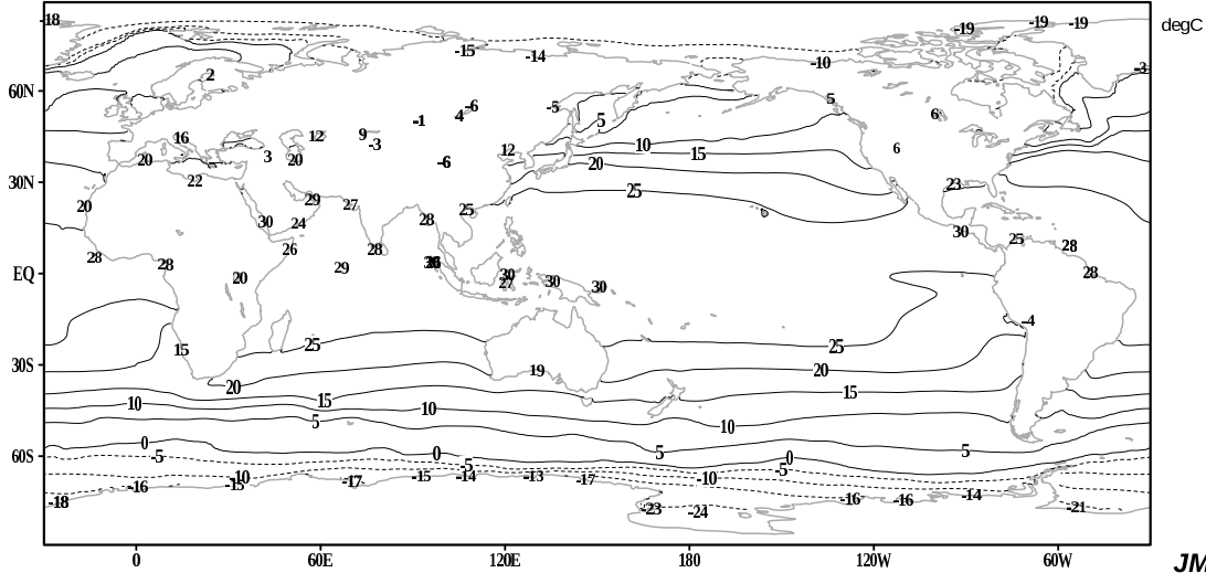
Sea surface temperature and sea ice surface temperature average (1981-2010) JMA December-February
